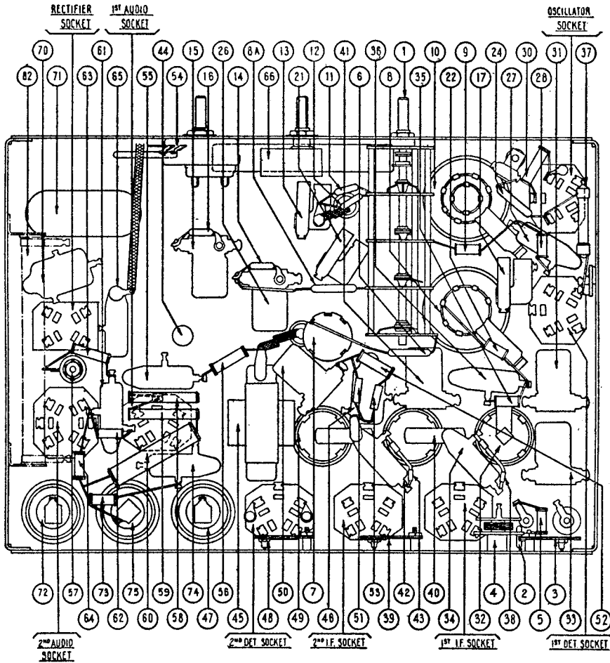
Fig. 3—Parts Diagram
